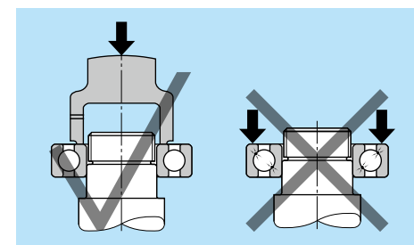
Fig. 15.11 Press-fitting bearing into shaft
