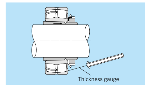
Fig. 15.24 Internal clearance measurement method for spherical roller bearings
