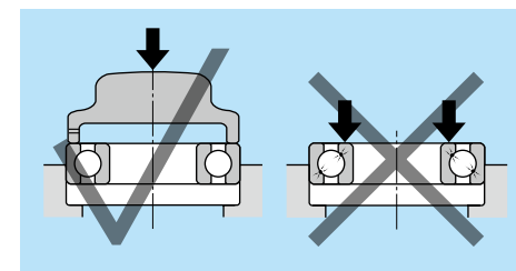
Fig. 15.12 Press-fitting bearing into housing
