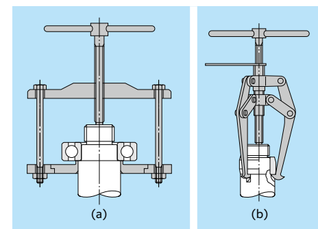
Fig. 15.28 Puller disassembly
