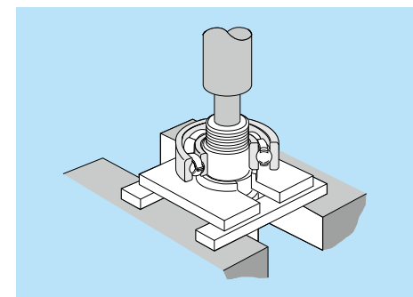
Fig. 15.29 Press disassembly
