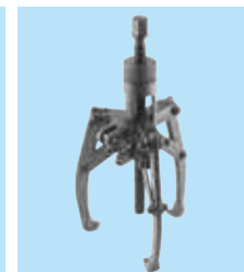
Fig. 15.47 Mechanical puller
