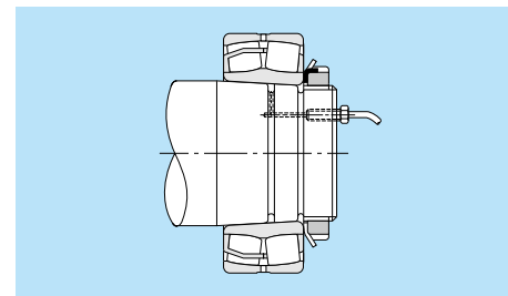
Fig. 15.21 Bearing installation using oil pressure
