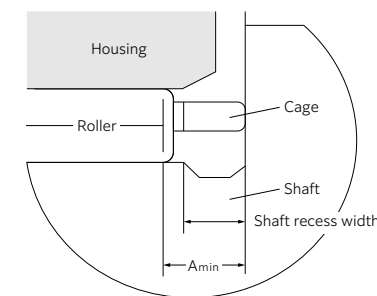
Fig. 1 Dimension A_{min}
