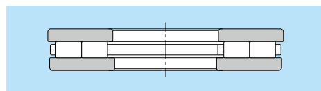
Fig. 3 Double row thrust cylindrical roller bearings
