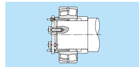
Fig. 15.23 Installation using hydraulic withdrawal sleeve
