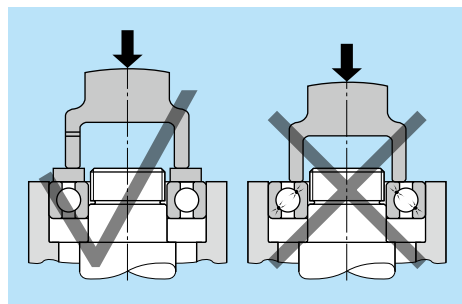
Fig. 15.13 Simultaneous press-fitting
