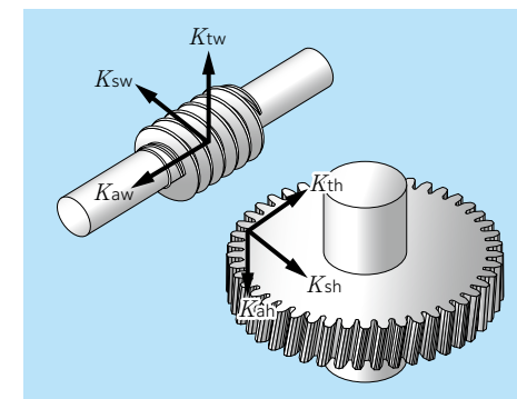
Fig. 4.7 Worm gears
