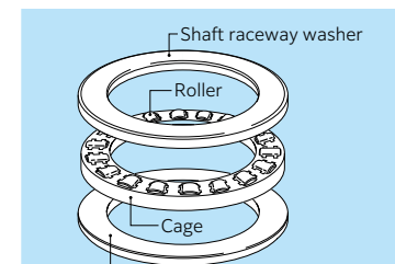
Fig. H Thrust roller bearing
