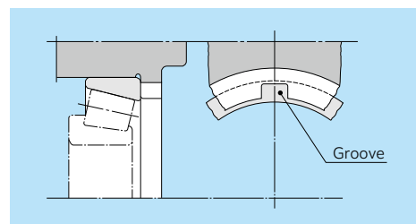
Fig. 15.31 Extraction groove for outer ring disassembly
