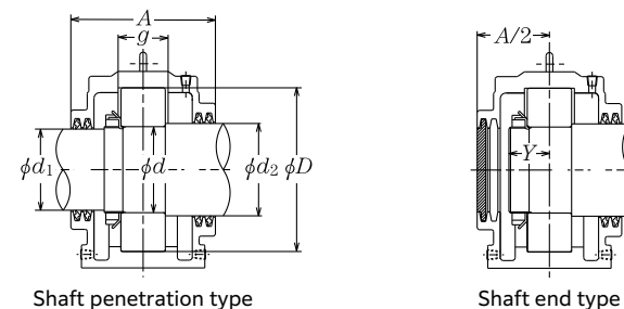
Shaft penetration type
