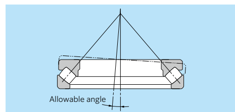
Fig. 2 Thrust spherical roller bearings
