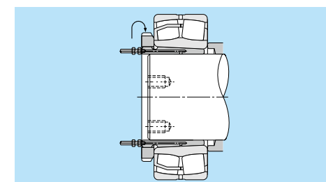
Fig. 15.39 Disassembly using hydraulic withdrawal sleeve
