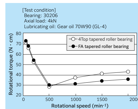
Fig. 13.8 Result of rotational torque measurement
