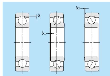
Radial internal clearance = \delta axial internal clearance \cong \delta_1 + \delta_2
