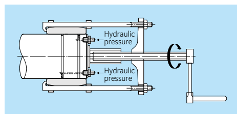
Fig. 15.33 Removal of bearing by hydraulic pressure
