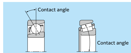
Fig. 1.3 Contact angle
