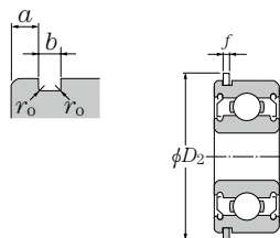
Shielded type with snap ring (ZZ)
