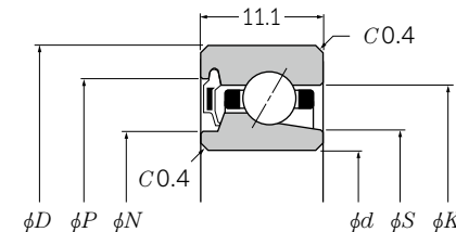
Angular type (with single-seal)
