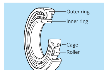
Fig. C Cylindrical roller bearing
