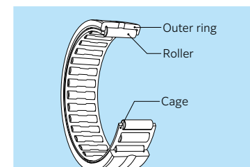
Fig. D Needle roller bearing
