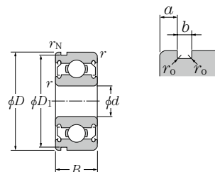
Shielded type with snap ring groove (ZZ)
