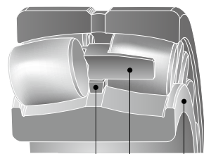
Guide ring One-piece machined cage Inner ring flange
