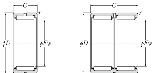
RNA48 type RNA49·R type RNA59 type NK·R type
