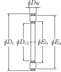
811 type, 812 type (Thrust cylindrical roller and cage assembly)
