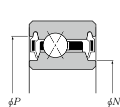
4-point contact type (with double-seal)
