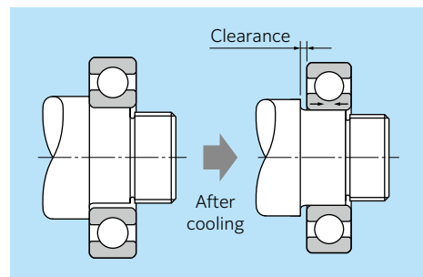
Fig. 15.19 Bearing contraction after heating
