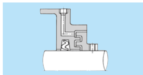
Fig. 8 Combination seal
