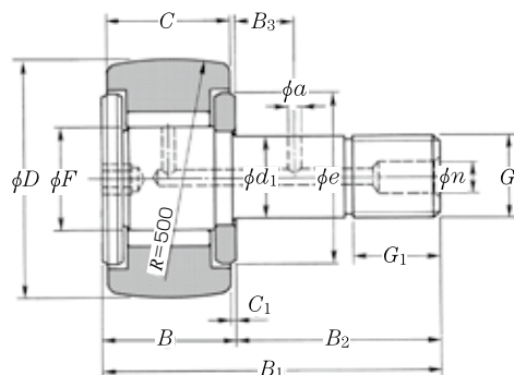
KRV···H type (Full complement roller type)
